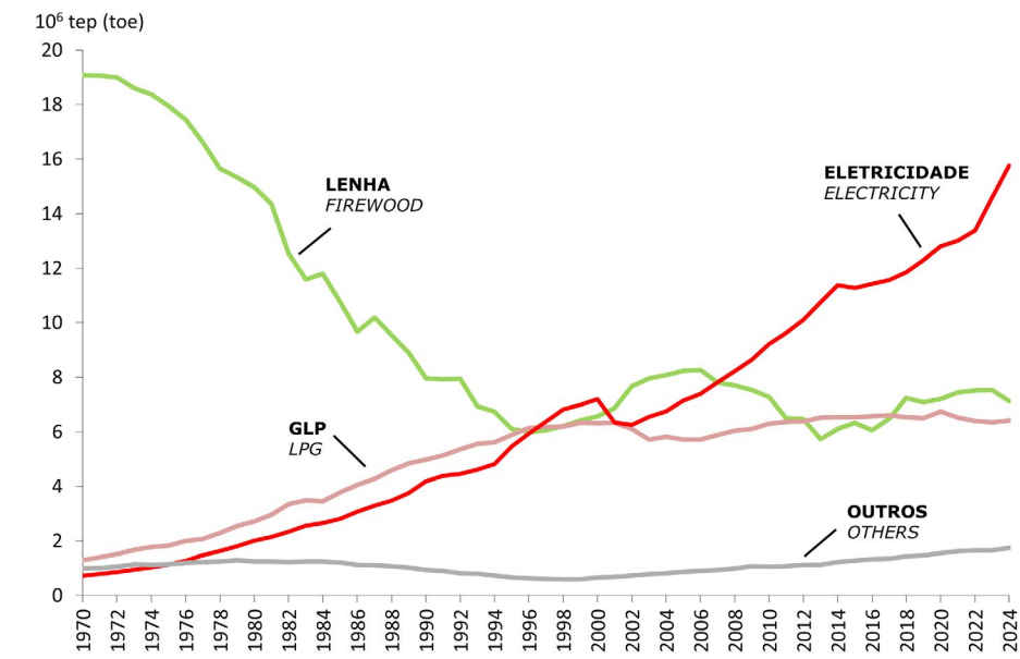
Gráfico 3.2 – Consumo Final no Setor Residencial Chart 3.2 – Residential Sector Energy Consumption
