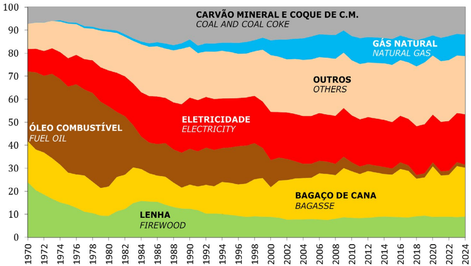
Chart 3.5 – Industrial Sector Energy Consumption
