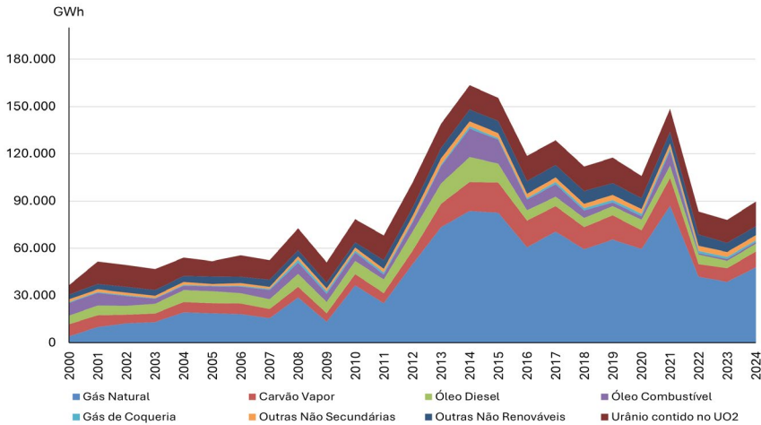
Chart 1.1.a - Electricity generation: non-renewable sources
