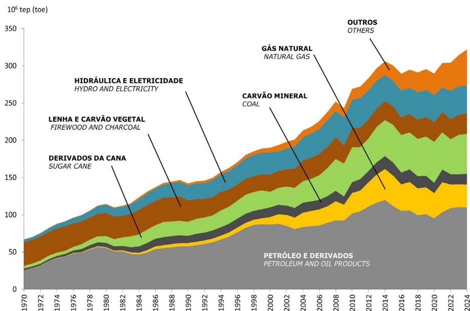
Chart 1.3.a – Domestic Energy Supply
