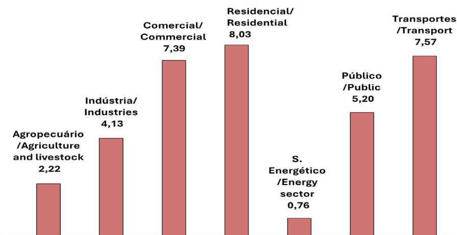
Chart 1.1.1 – Percentual Change of Electricity Consumption per Sector
