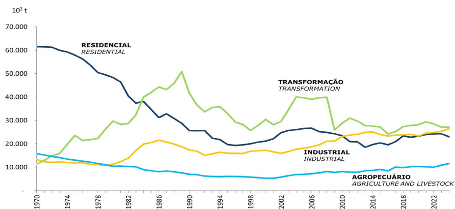
Chart 2.4 – Firewood
