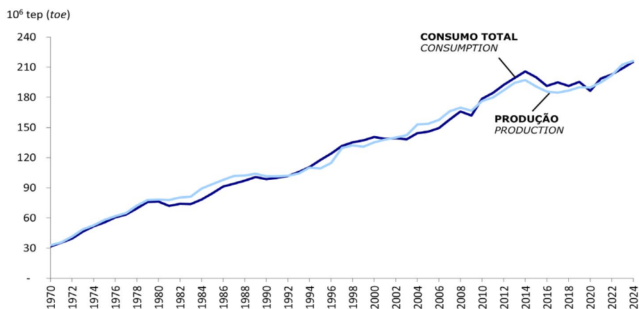
Chart 2.5 – Secondary Sources
