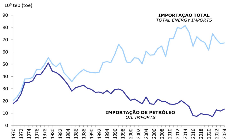
Chart 4.3 – Energy Imports
