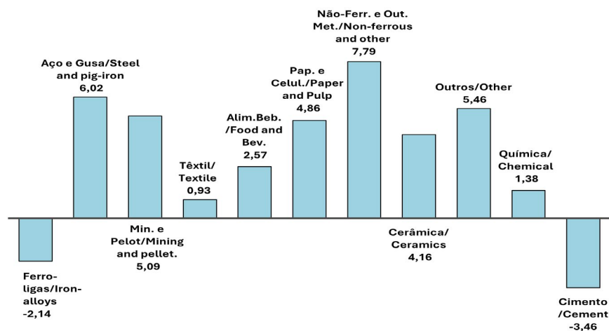
Chart 1.1.2 – Growth of Electricity Consumption in the Industrial Sector
