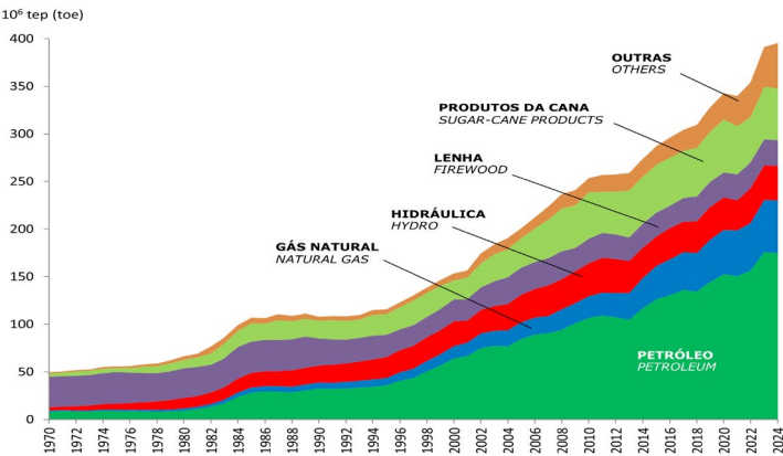
Chart 1.2.a – Primary Energy Production
