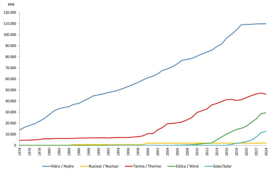
Chart I.1 – Installed Capacity Of Electric Energy Generation
