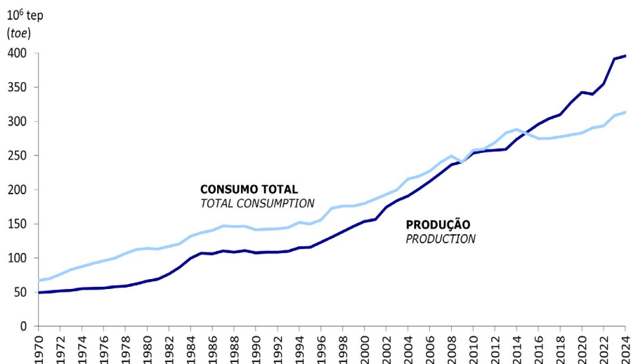
Chart 2.1.b – Primary Energy
